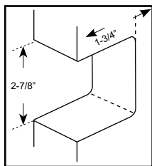
Notching Dimensions
