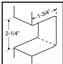
Notching Dimensions
