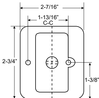
Notching Dimensions
