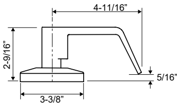
Latch: 1-1/8"x2-1/4" square corner, 2-3/4" backset, UL Strike: FASA: 1-1/4"x4-7/8", square corner
